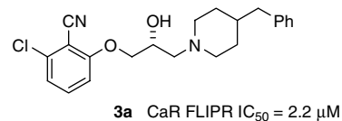
Figure 2. Hit from library.
