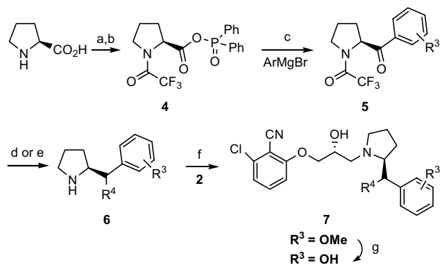
Scheme 2. Reagents and conditions: (a) \text{CF}_3\text{CO}_2\text{Et} , 1,1,3,3-tetramethylguanidine, 82%; (b) \text{ClP(O)Ph}_2 , \text{NEt}_3 , 79%; (c) THF, -70^\circ\text{C} to rt, 17–60%; (d) \text{H}_2/\text{Pd/C} , EtOH, HCl, 48 h, 100%; (e) (i) \text{BF}_3\cdot\text{OEt}_2 , \text{Et}_3\text{SiH} , 41–55%; (ii) 12.5 N HCl, i -PrOH reflux, 100%; (f) EtOH, 110^\circ\text{C} , 16 h, 47–55%; (g) \text{BBr}_3 , \text{CH}_2\text{Cl}_2 , -70^\circ\text{C} to rt, 80%.
