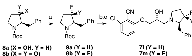
Scheme 3. Reagents and conditions: (a) BAST, \text{CH}_2\text{Cl}_2 , -78^\circ\text{C} to rt, overnight, 23% ( Y = \text{H} ), 72% ( Y = \text{F} ); (b) TFA, \text{CH}_2\text{Cl}_2 ; (c) 2 , 90^\circ\text{C} , overnight, two steps 37% ( Y = \text{H} ), 74% ( Y = \text{F} ).
