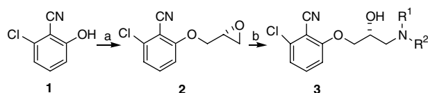
Scheme 1. Reagents and conditions: (a) ( R )-epichlorohydrin, \text{Cs}_2\text{CO}_3 , \text{CH}_3\text{CN} , reflux overnight, 84%; (b) i -PrOH, \text{NHR}^1\text{R}^2 , 80 °C, overnight, 8–100%.
